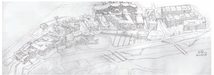
Drawing for the Xiangshan Campus of the China Academy of Art (Phase II) , 2005. 64.9×22.8cm Pencil on paper
